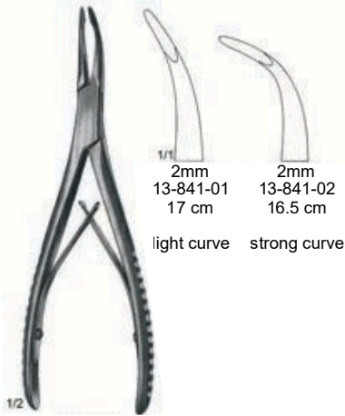
Stellbrink 13-841-01 - 13-841-02
